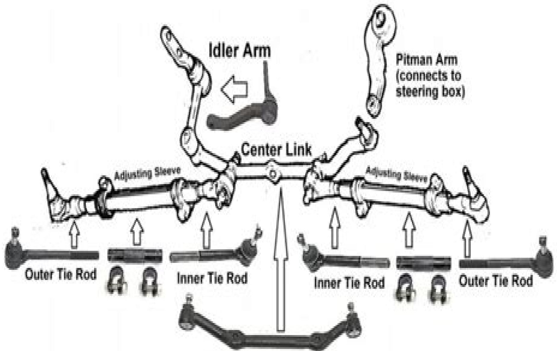
Parallelogram Steering
